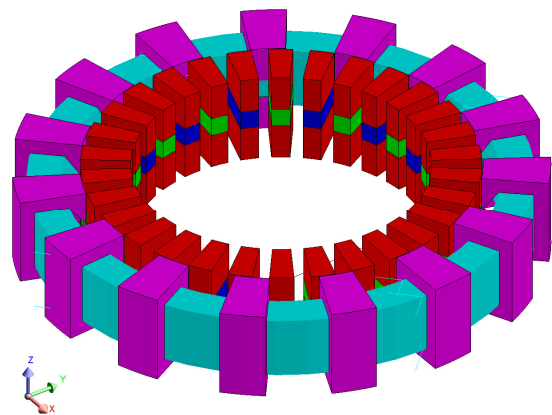
Fig. 2 3D view of the PMTFG phase module
