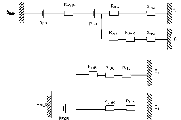
Fig. 6 PMTFG thermal equivalent circuits a) heat transfer from stator to rotor and exterior b) heat transfer from rotor to stator and air-gap
