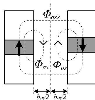
Fig. 4 Rotor pole, side and side to side leakage flux
