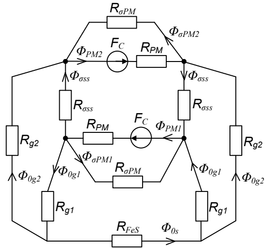
Fig. 3 Magnetic equivalent circuit at no load ( I=0 )
