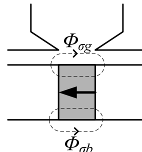
Fig. 5 Rotor PM's air-gap and bottom leakage flux
