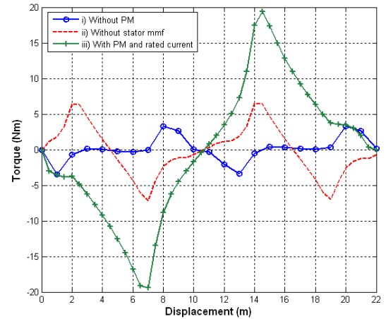
Fig. 8 PMTFG torque per module versus rotor displacement
