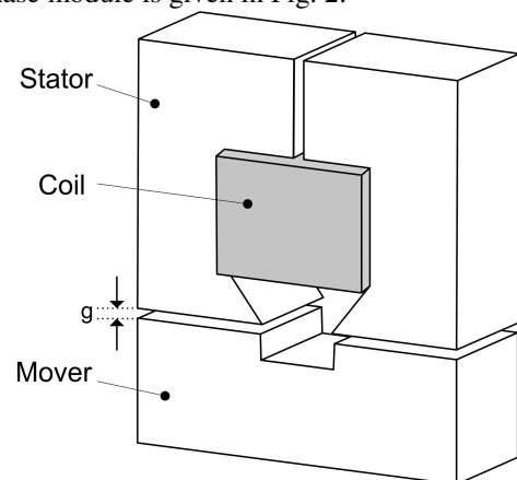
Fig. 1 A basic structure of a TF reluctance machine
