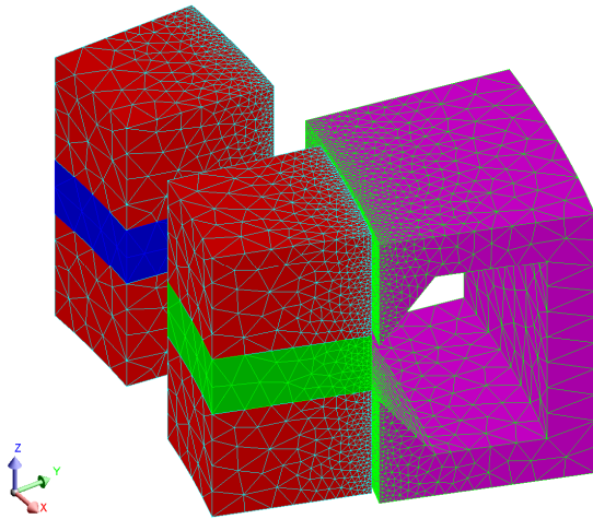
Fig. 7 PMTF machine meshing
